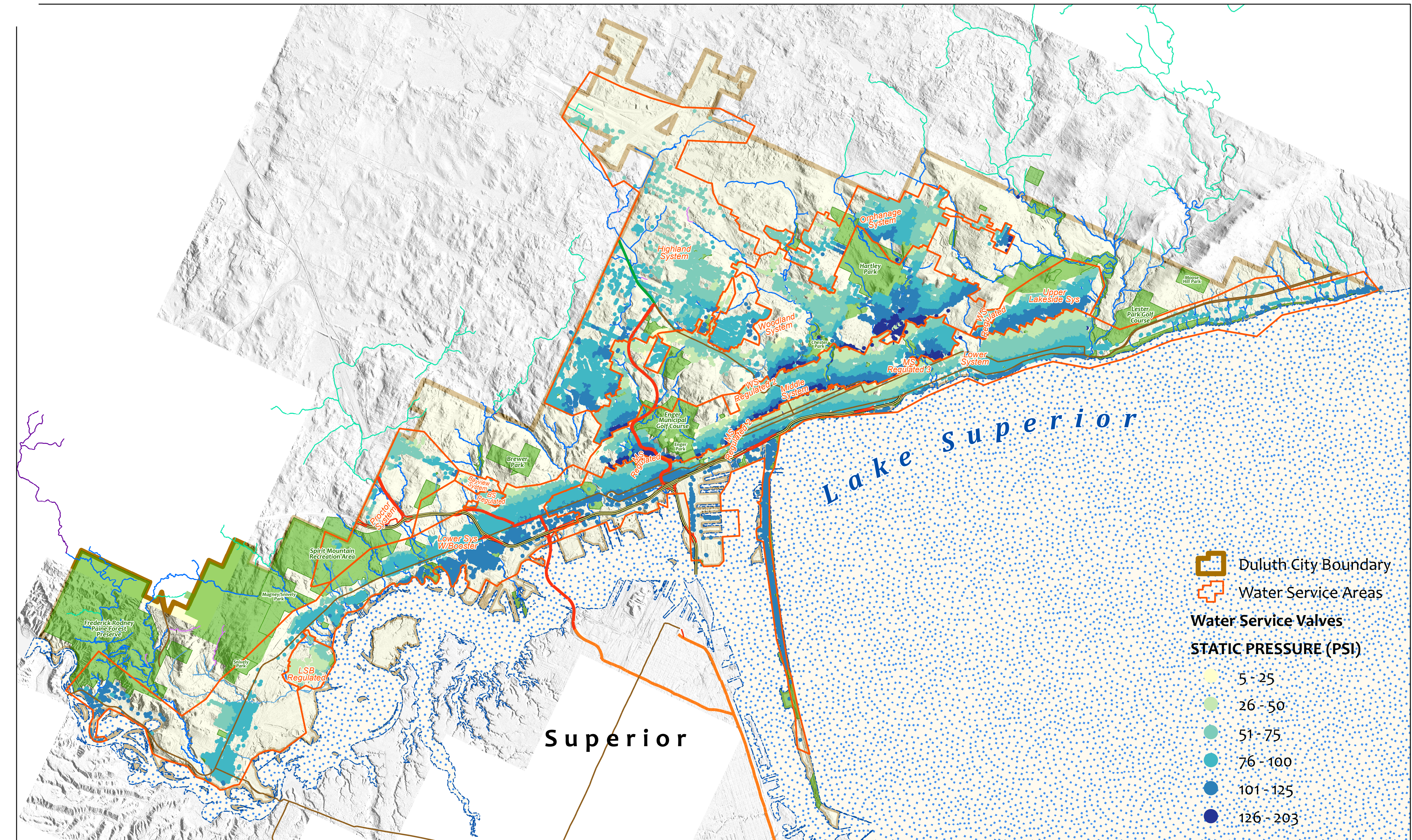
Water Service Valve Static Pressure
